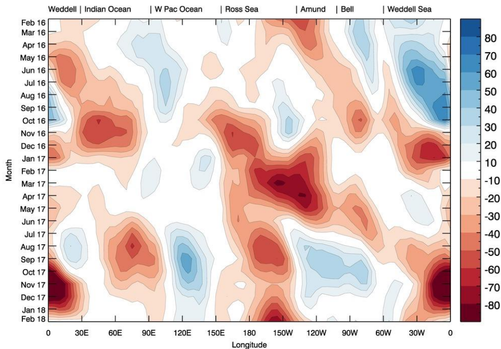
Figure 2. Hovmöller (longitude-time) diagram of Southern Ocean sea-ice extent anomalies relative to the 1981-2010 climatology (km 2 per 5° longitude).
