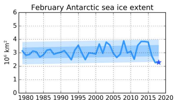
Figure 1. February Antarctic sea-ice extent (Fetterer et al., 2017). The star is February 2018. The dashed line is the linear trend and the two shaded intervals show 1 and 2 standard deviations of the residuals around the linear fit, respectively
