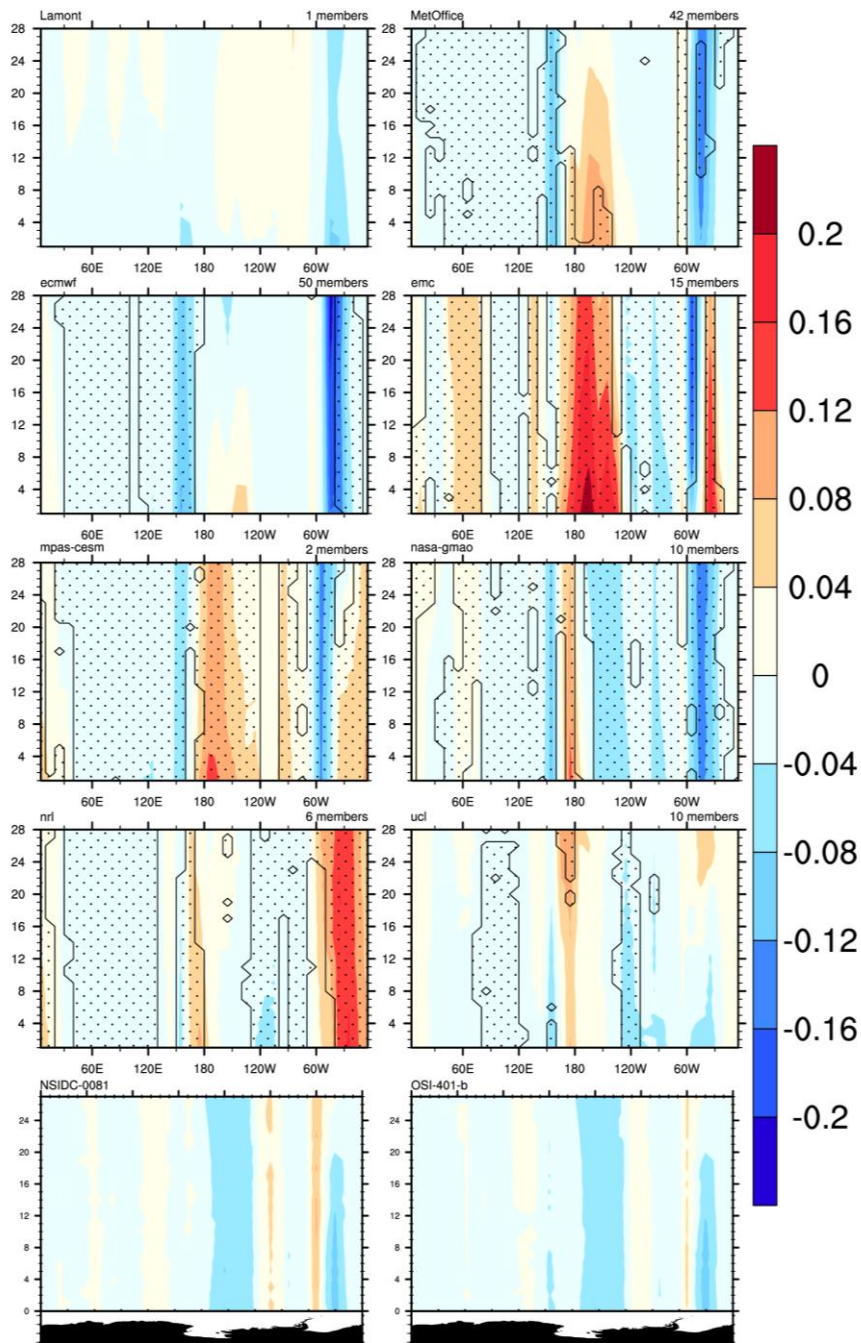
Figure 6. Ensemble-mean predicted daily rSIA anomaly (compared to 1979-2014 NASA Team SIC climatology) for February 2018 [ 10^6 km 2 ] as a function of longitude (horizontal dimension) and time in February (vertical dimension). For submissions with an ensemble of members, hatching indicates where the sign of the predicted anomaly agrees across all the submission members.
