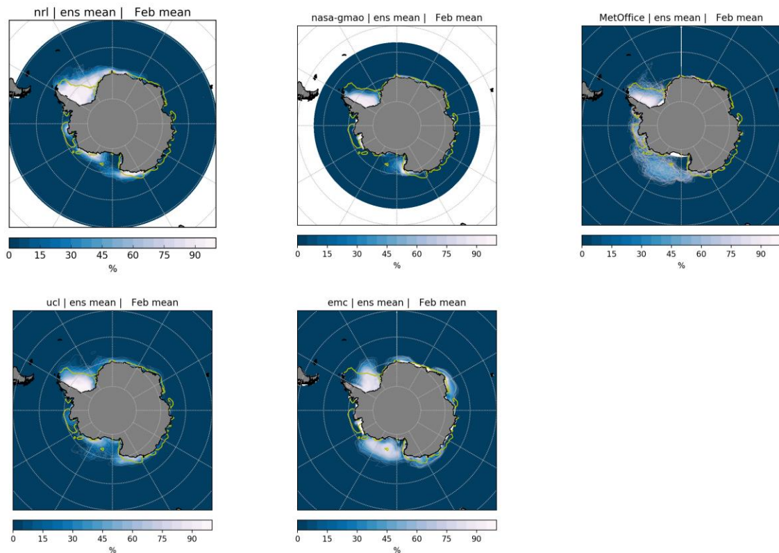
Figure 7. Ensemble mean of February 2018 monthly mean sea-ice concentration, as forecast by the five groups that contributed daily sea-ice concentration information. The thin lines are the ice edge position for each forecast member, determined as the 15% contour line of the monthly mean sea ice concentration for the member. Yellow lines are the 15% contours of monthly mean sea-ice concentration from the two observational references OSI-401-b and NSIDC-0081.
