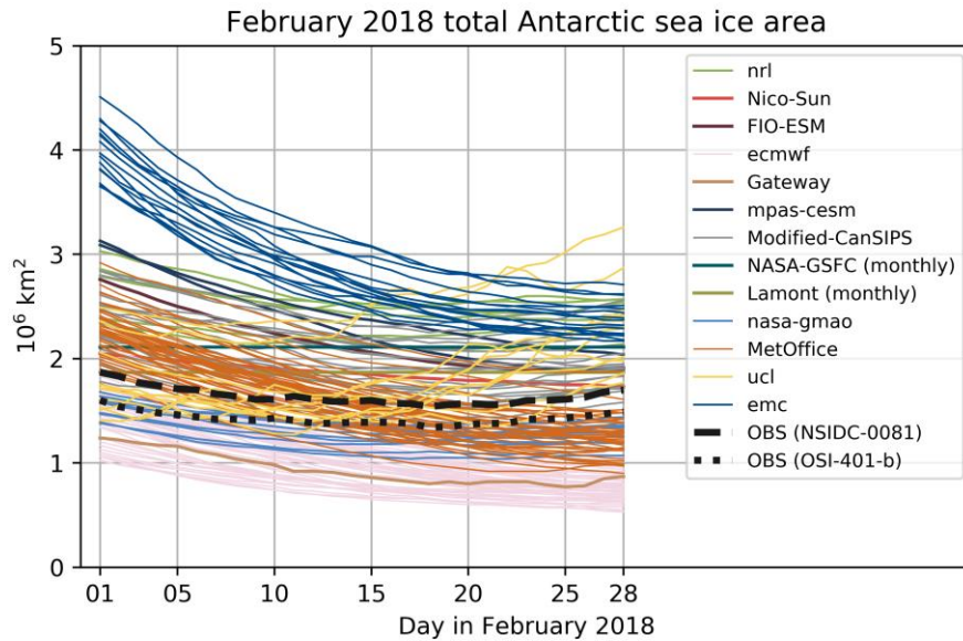
Figure 3. Total (circumpolar) Antarctic sea-ice area of the 13 forecasts for each day of February 2018. The black dashed lines are two observational references (Maslanik and Stroeve, 1999 and Tonboe et al., 2017).
