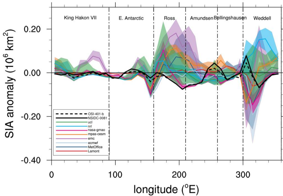
Figure 5. February 2018 mean rSIA anomaly (compared to 1979-2014 NASA Team climatology) by longitude, for each submission, with observed estimates given in black. Solid lines show the ensemble mean for each contribution, with transparent shading indicating the ensemble range (min-max).
