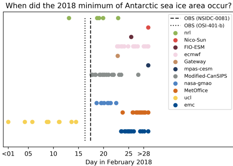
Figure 4. Timing of the seasonal (February) Antarctic minimum sea-ice area of the forecasts (monthly mean forecasts are discarded), along with two observational references (Maslanik and Stroeve, 1999 and Tonboe et al., 2017). To filter the effects of synoptic variability on total sea-ice area, the minimum was determined from a quadratic fit of the daily sea-ice area time series.
