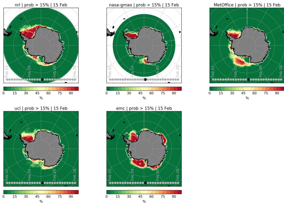
Figure 8. Probability of sea-ice presence for 15 th February 2018, as forecast by the five groups that submitted daily sea-ice concentration information. The sea-ice edge as observed by two products (OSI-401-b and NSIDC-0081) is shown in white. The probability of presence for a given day corresponds to the fraction of ensemble members that simulate sea-ice concentration larger than 15% in a given grid cell, for that day. A dynamic animation of the figure showing all 28 days of February is available at http://acecrc.org.au/sign-south/ .
